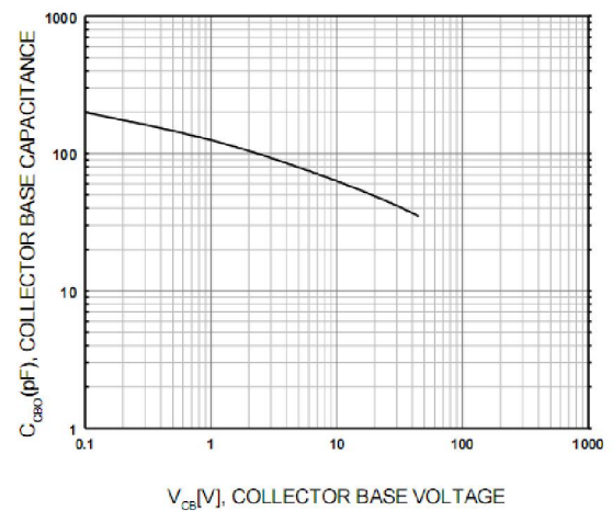
Figure 4. Collector-Base Capacitance
