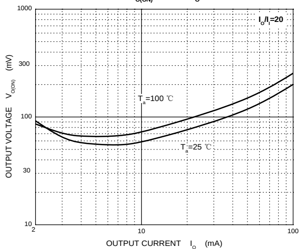
V_{O(ON)} - I_O
