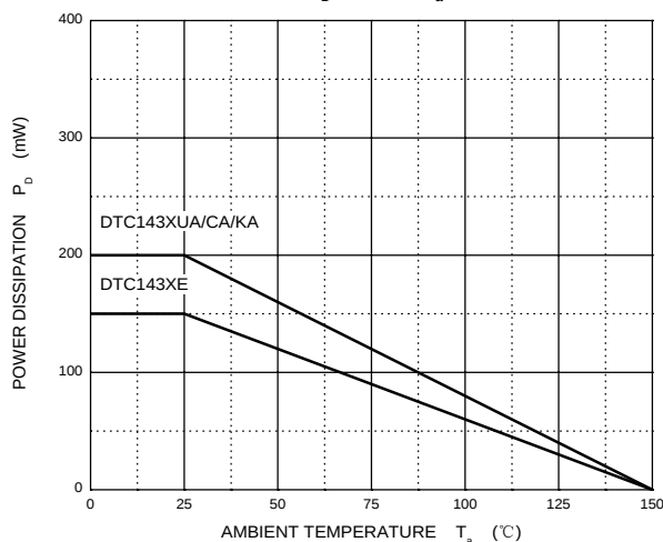
P_D - T_a
