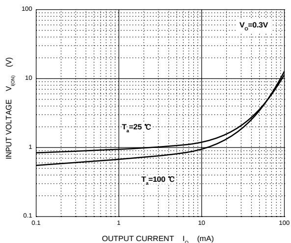
ON Characteristics
