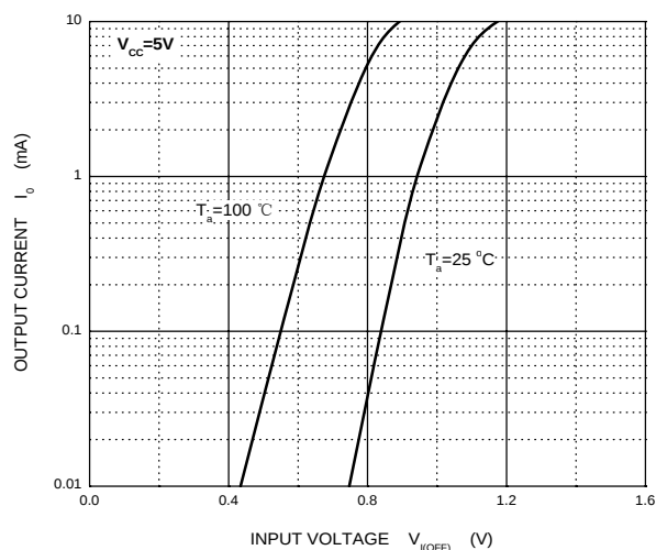
OFF Characteristics
