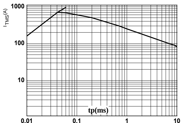
FIG.5: Non-repetitive surge peak on-state current for a sinusoidal pulse with width t_p < 10ms
