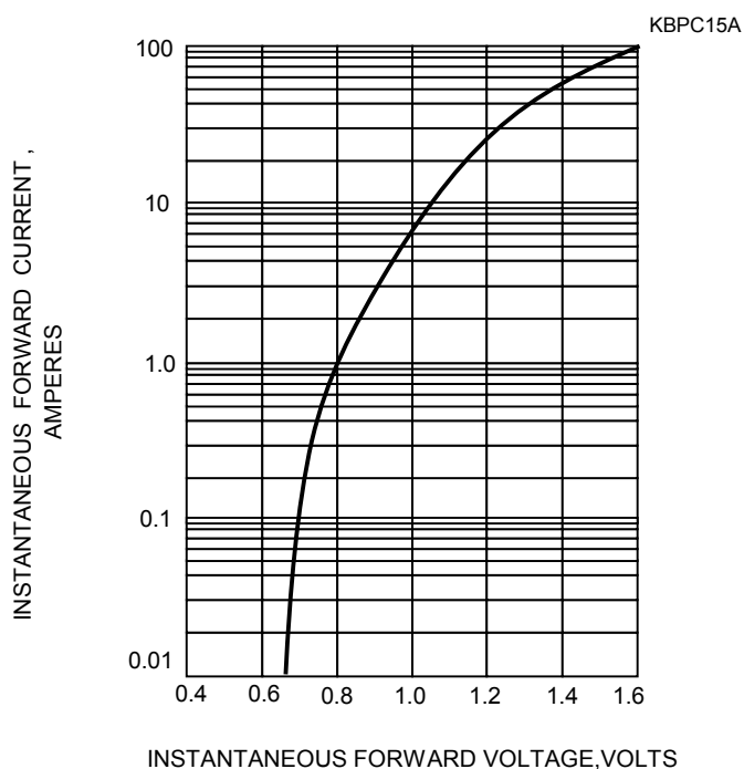
FIG.3-TYPICAL FORWARD CHARACTERISTICS
